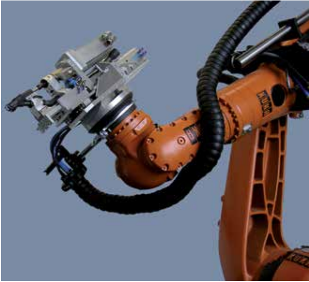
Robot-assisted fastening system supplied by Weber Schraubautomaten
