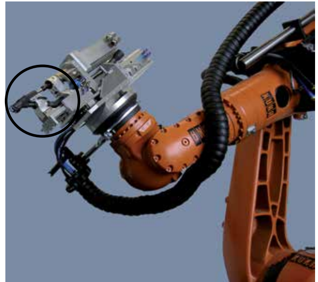
Robot supported fastening system of the company Weber Schraubautomaten.
